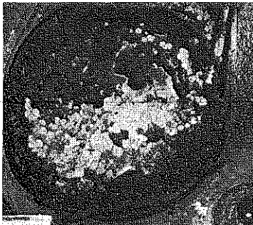
LEAD FOULING —Crusty lead deposits on pistons, after 42,168 miles running with a nationally-sold leaded premium gasoline.
